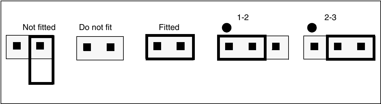
Figure 4. Jumper positions
